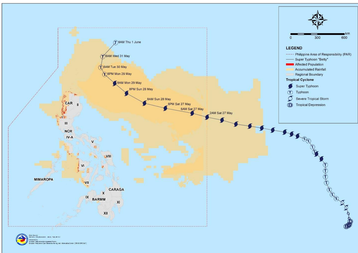
Figure 1. Accumulated Rainfall of at Least 100mm for the Next 120 Hours (GSM) and 150mm for the Next 72 Hours (WRF)
