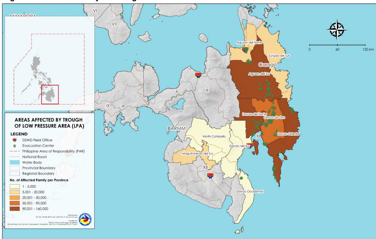
Figure 1. Areas affected by the Trough of LPA
